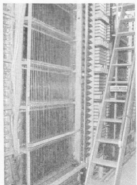
Western Electric Panel Switch, circa 1923 - believed to be the only working panel switch anywhere in the world
